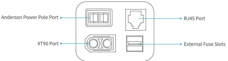
2/ Back Interface
