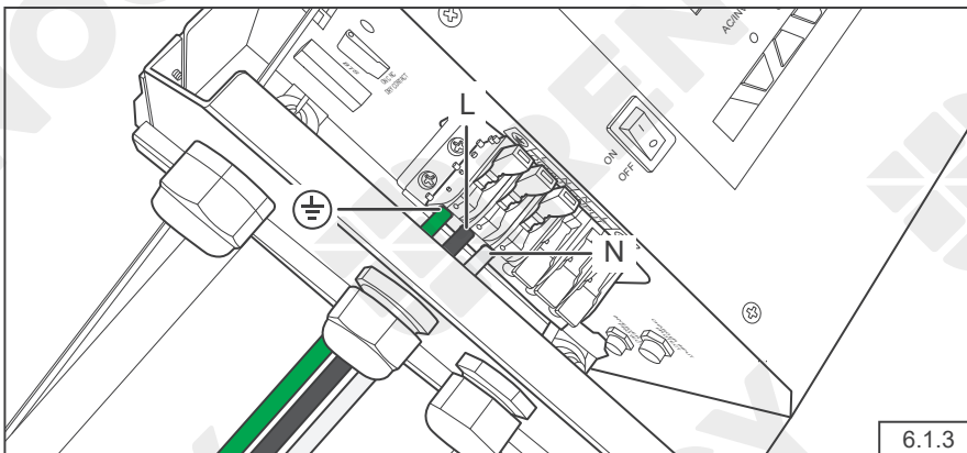
Connect the live wire to the (L) terminal hole, the neutral wire to the (N) terminal hole, and the ground wire to the (GND) terminal hole.
